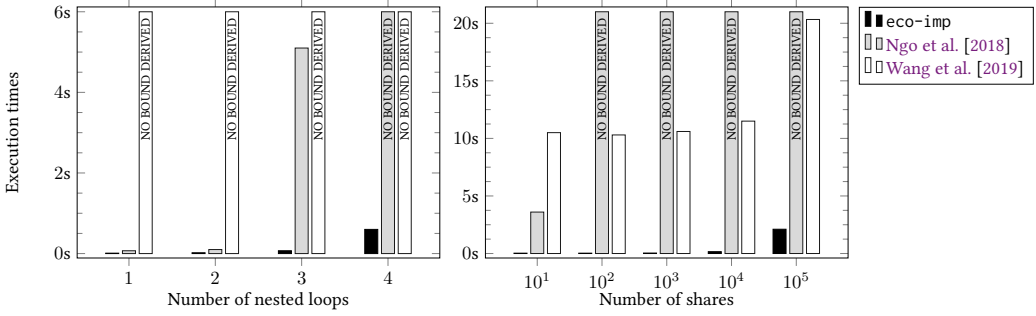
Fig. 8. Execution times of the three analysers on parametric examples (a) \text{nest-}i consisting of i nested loops, each performing a biased random walk and (b) \text{trader-}n from Figure 1a with number of shares fixed to n .
